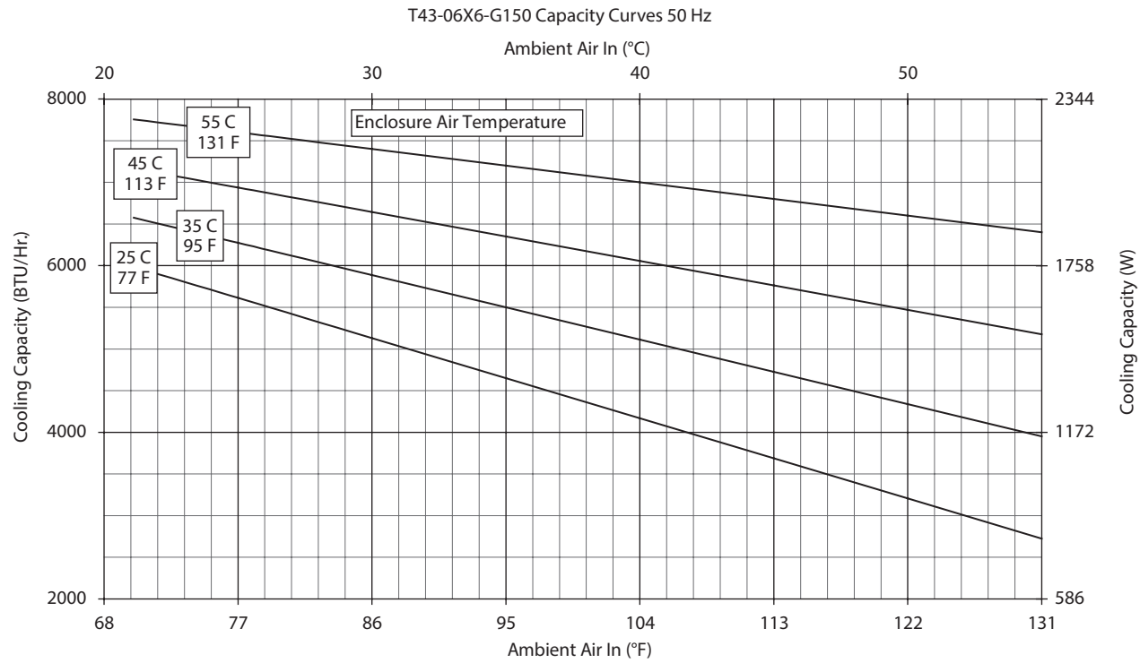
Performance Curves for T43 Models 6000 BTU/Hr. (1758 Watt)
