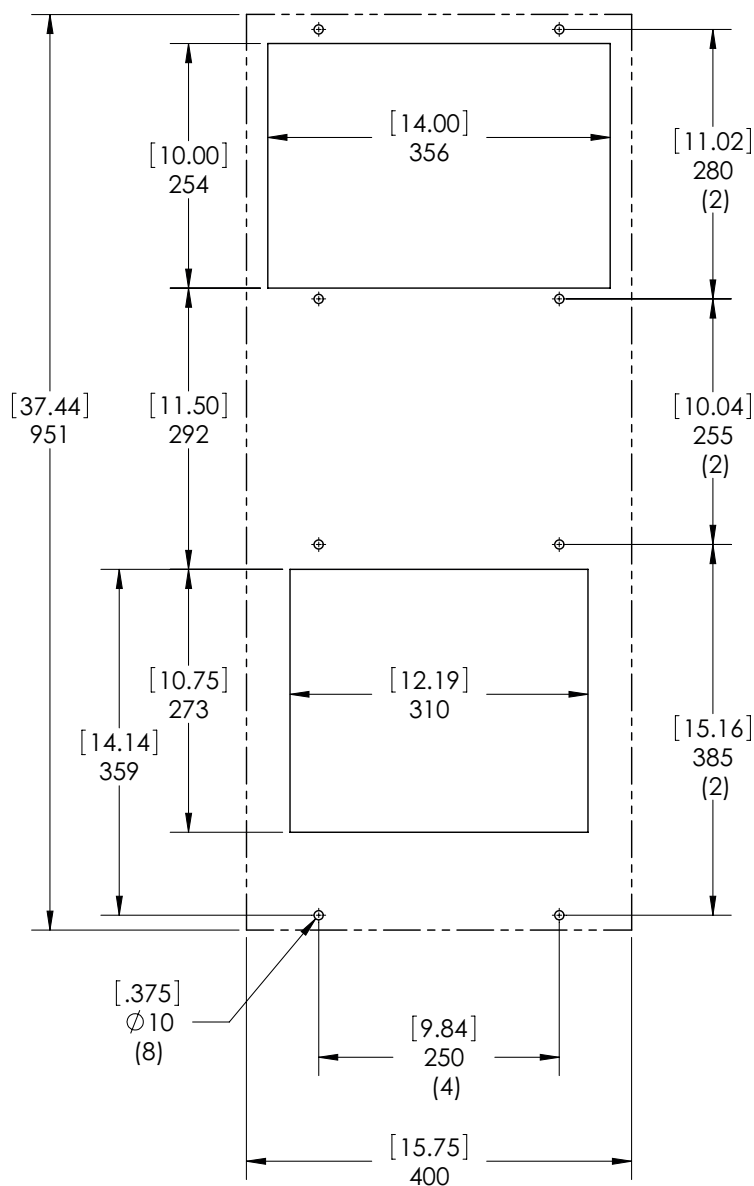
Surface Mount
