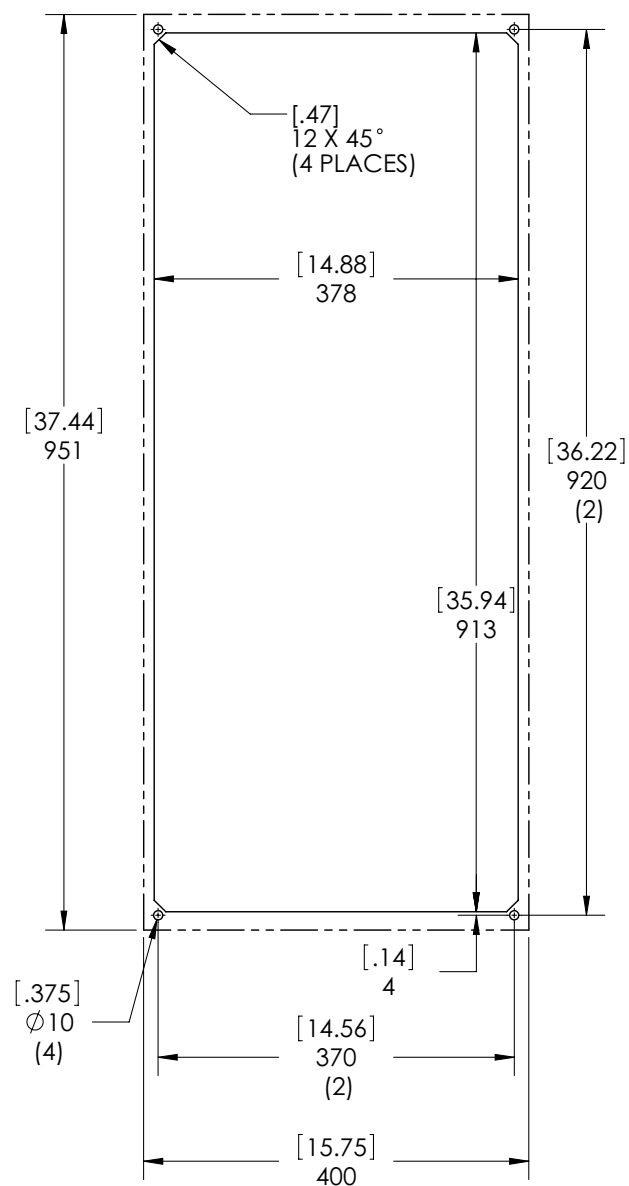
Partial and Full Recess Mount
