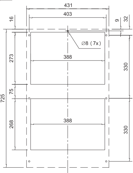
Cutout Dimensions External Surface Mount
